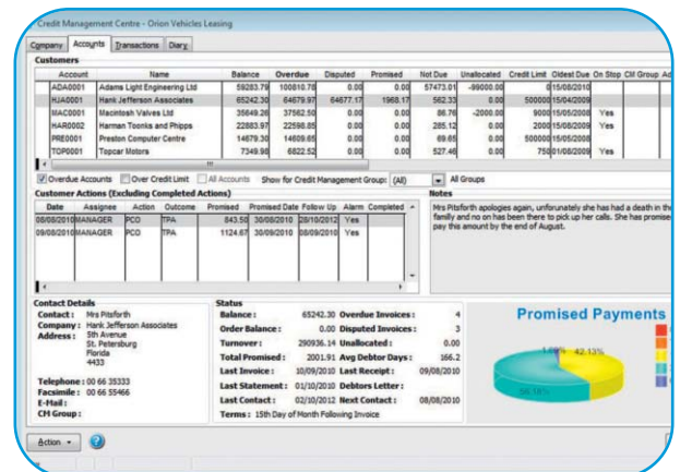
Accounts view
